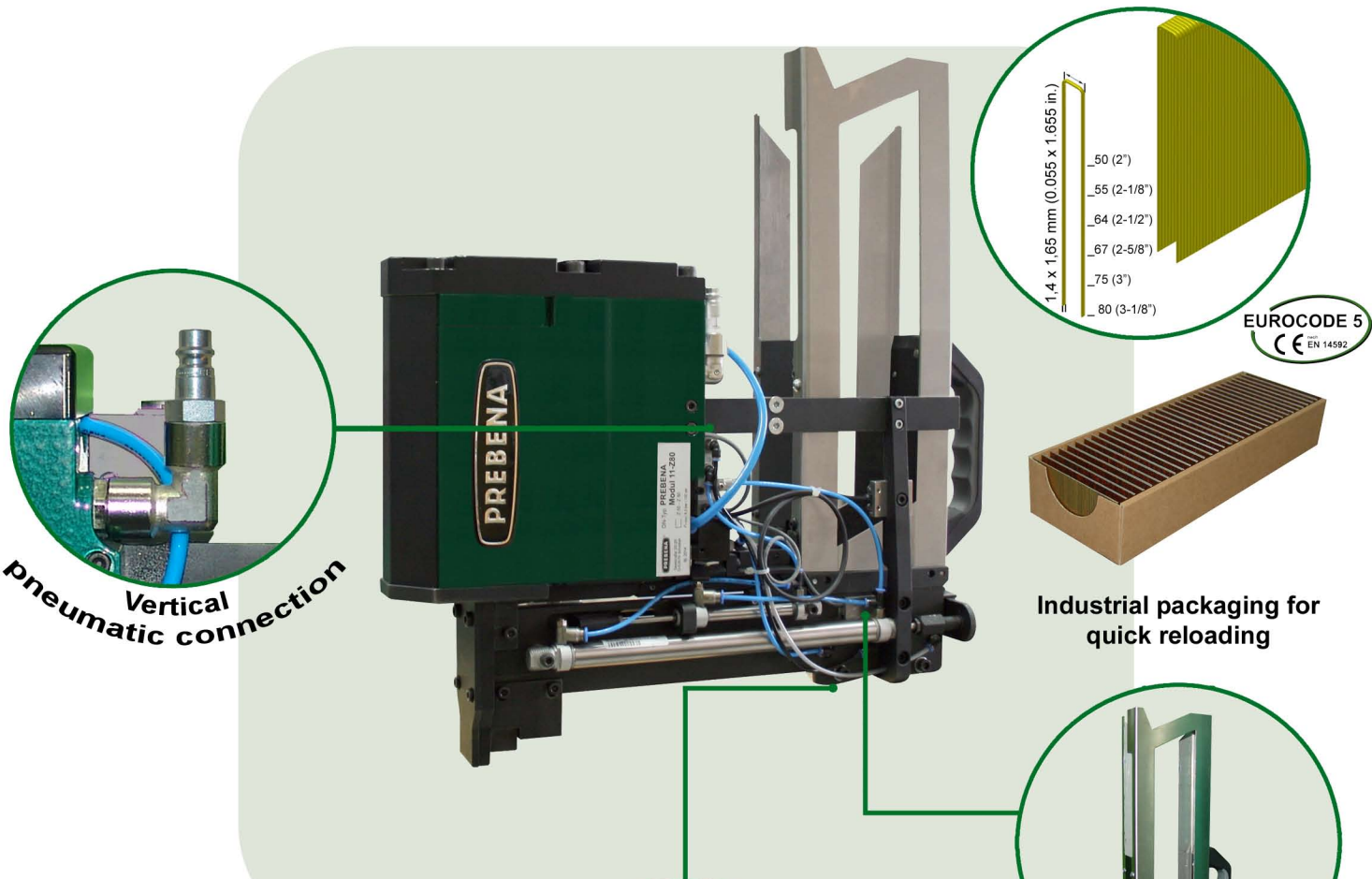
Changeable magazine for easy and quick loading
